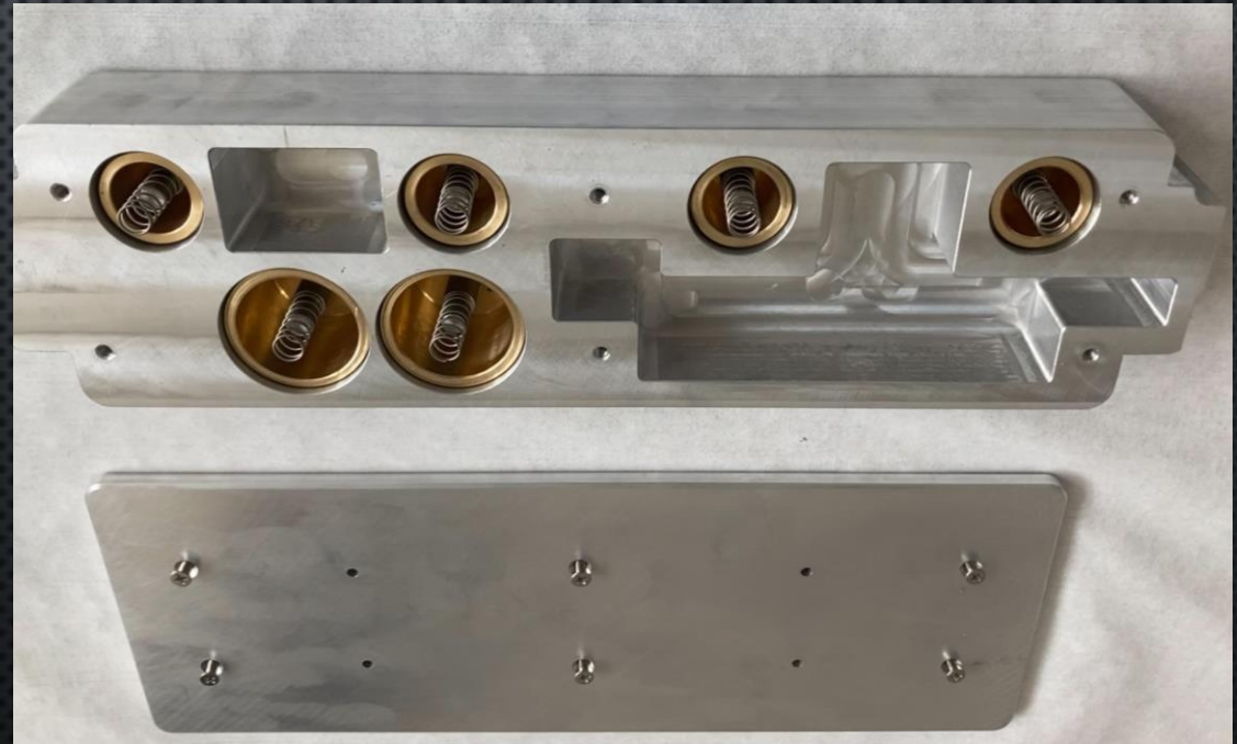
Assembly fixture
