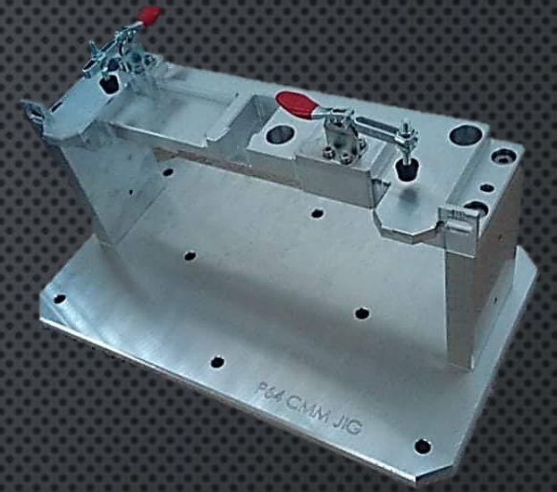
CMM support fixtures
